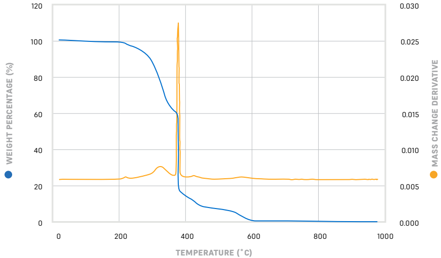
True Cast Resin TGA Trace
